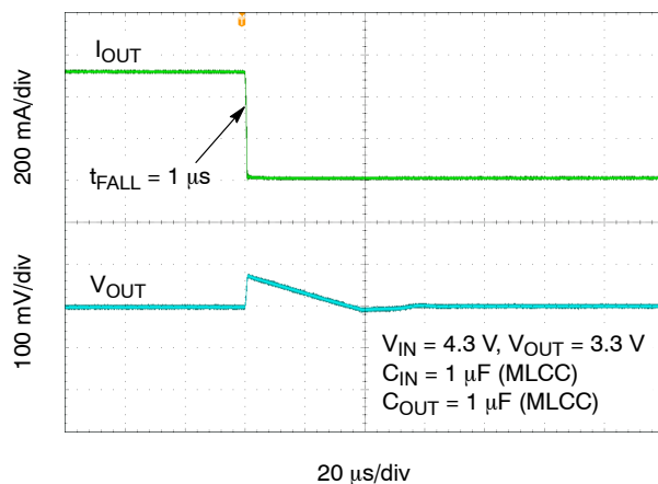
Figure 35. Load Transient Response – 450 mA to 1 mA – V_{OUT} = 3.3 \text{ V}
